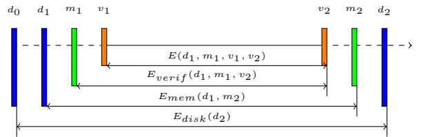
Figure 1: Without partial verifications.
